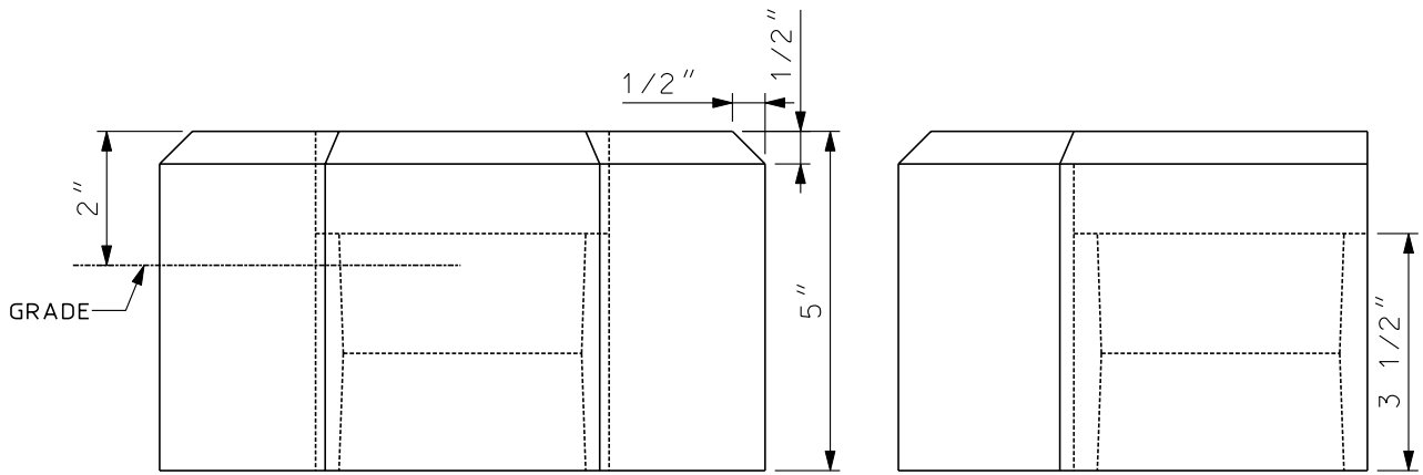
SIDE ELEVATION
