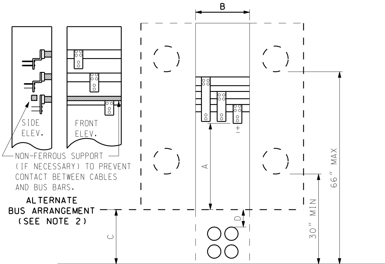
FIGURE 2. MULTI-METER BANKS (LIMITED TO 6 METERS MAX.) DUCTS IN WALL DIRECTLY BELOW CABLE COMPARTMENT.
