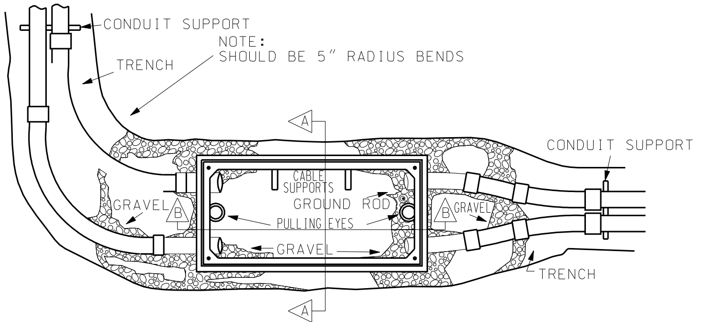
PLAN VIEW OF SPLICE BOX
