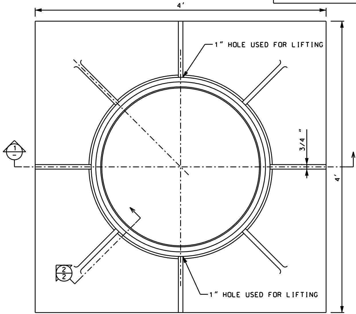
PLAN VIEW
