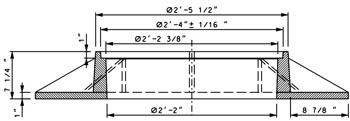
SECTION 1
