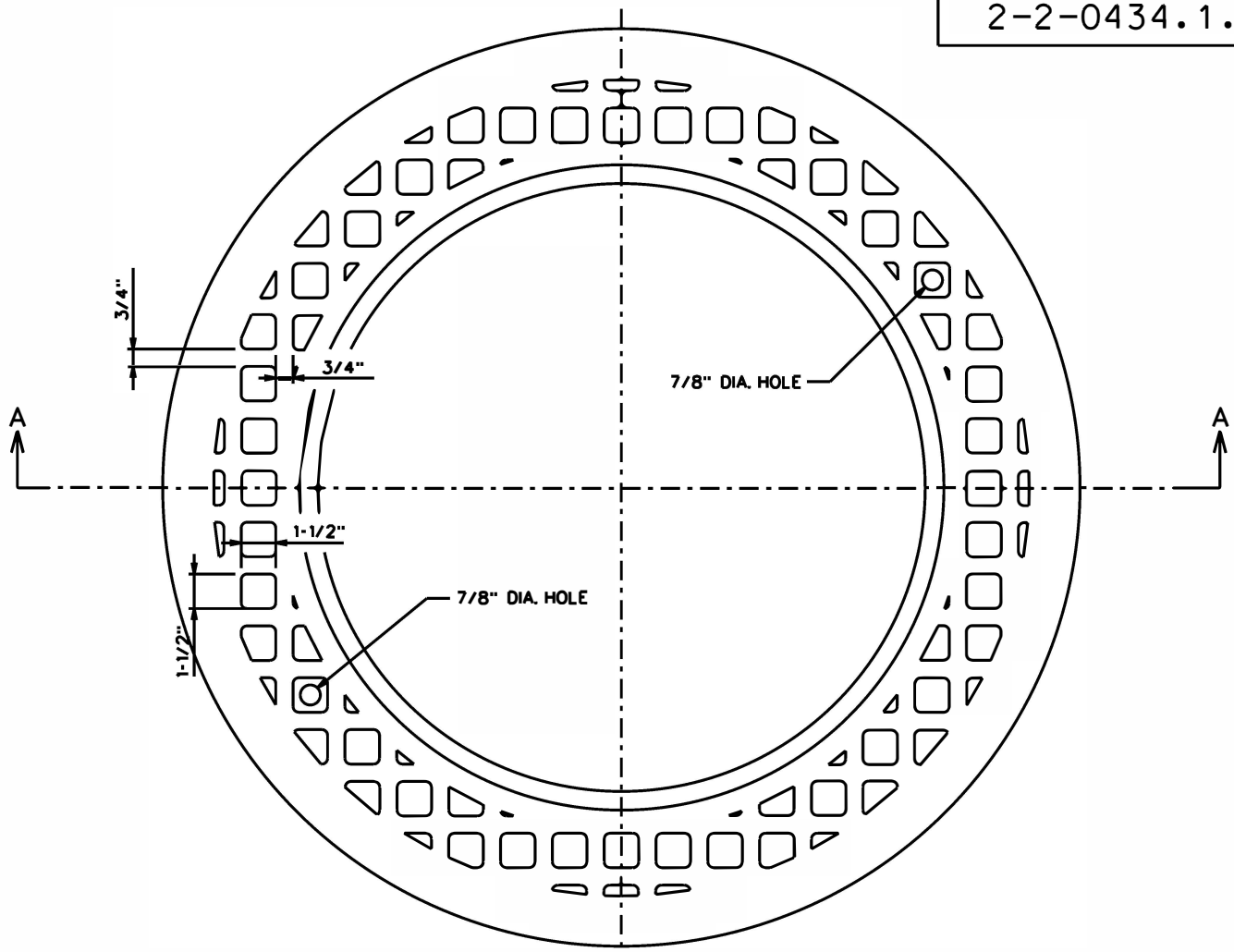
TOP VIEW
